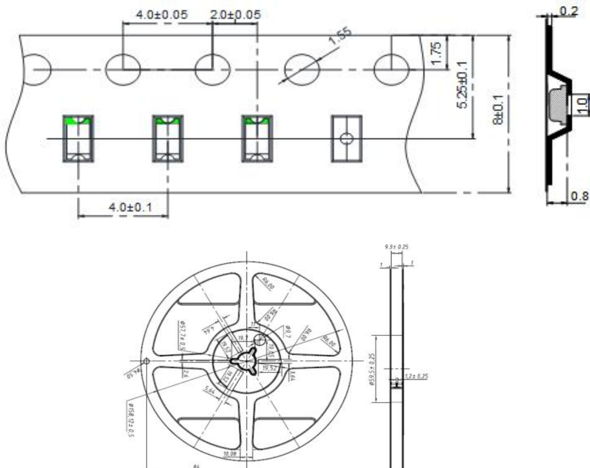
载带与圆盘尺寸 Belt and disk dimensions
