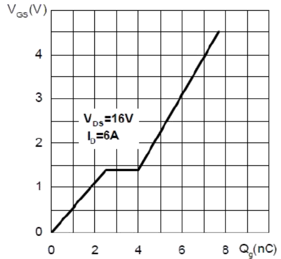
Figure 8 Gate Charge
