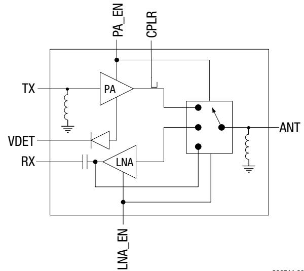
Figure 1. SKY85797-11 Block Diagram
