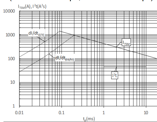
FIG.6: Non-repetitive surge peak on-state current for a sinusoidal pulse with width t_p < 20\text{ms} , and corresponding value of I^2t (I - II: di/dt < 50\text{A}/\mu\text{s} ; III-IV: di/dt < 20\text{A}/\mu\text{s} )
