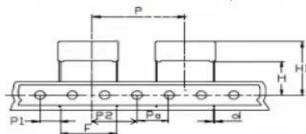
Fig 4 Pitch: 22.5/27.5 P_0=12.7
