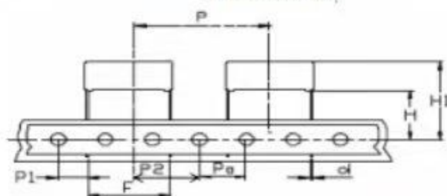
Fig 4 Pitch: 22.5/27.5 Po=12.7
