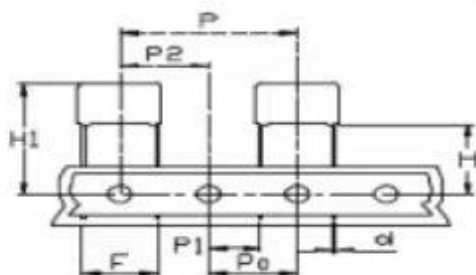
Fig 3 Pitch: 10/12.5/15 Po=12.7
