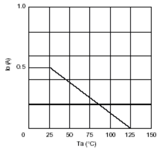
Fig.4 Derating curve
