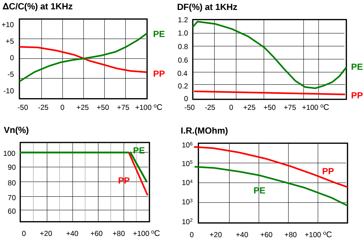
Temperature Characteristics
