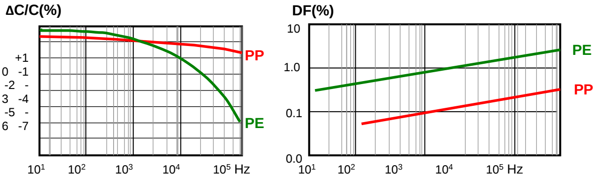
Frequency Characteristics
