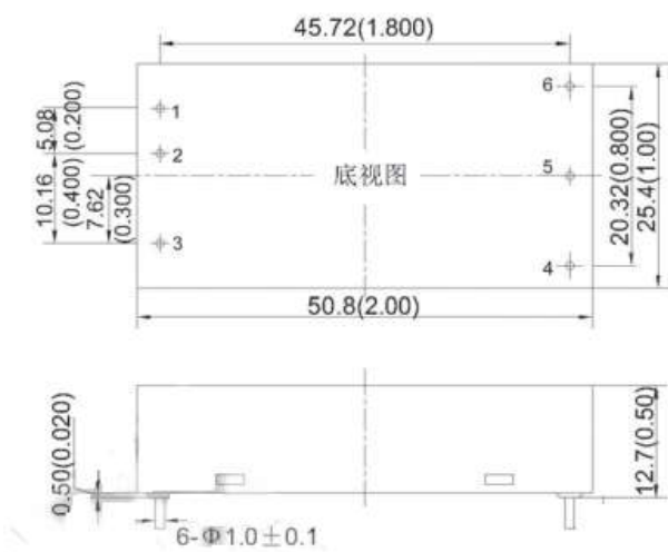
TDK30-XXSXX 尺寸图
