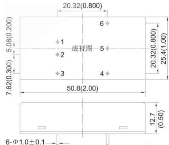
TDK30-XXSXXM 尺寸图
