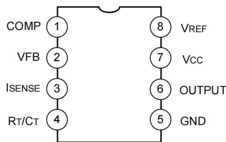
DIP-8/SOP-8
