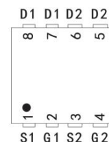
pin assignment
