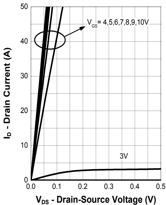
Output Characteristics
