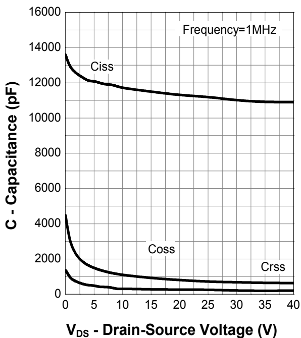
Capacitance
