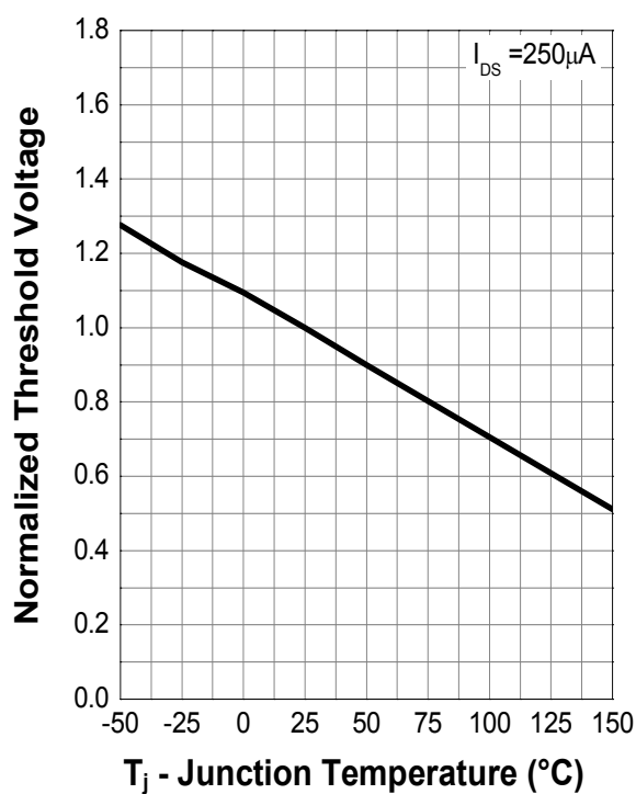
Normalized Threshold Voltage
