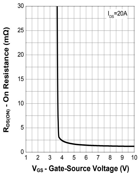
Transfer Characteristics
