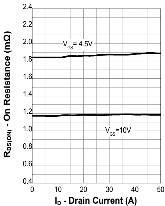
On Resistance
