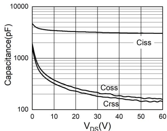
Figure 8. Capacitance
