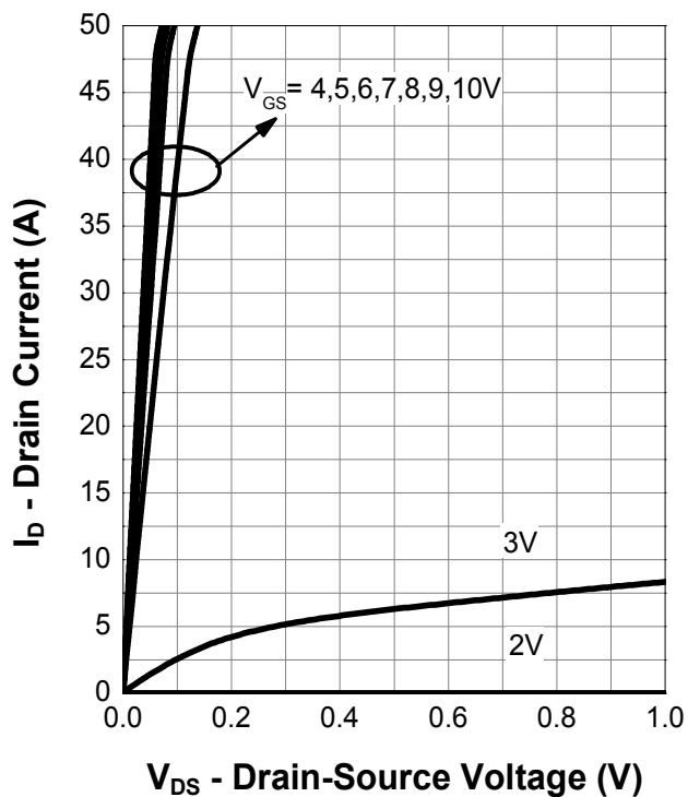
Output Characteristics
