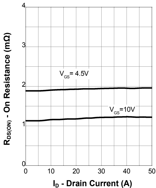
On Resistance
