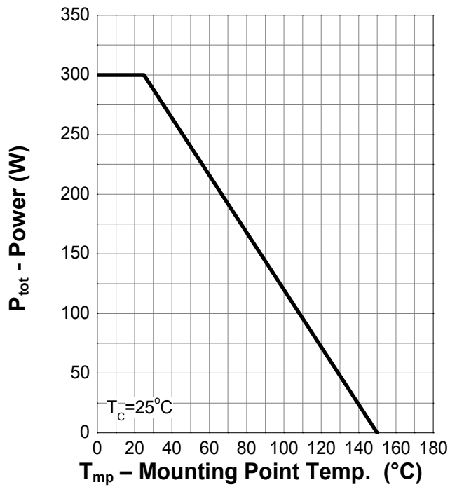
Power Capability
