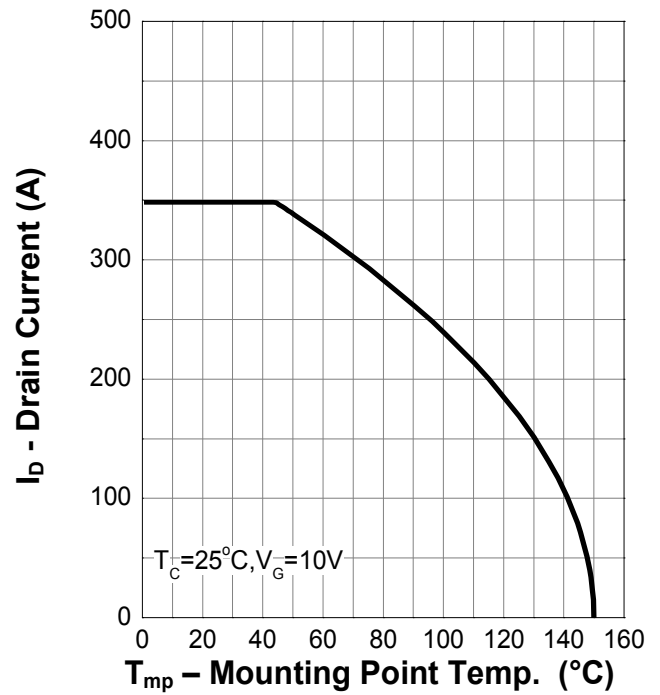
Current Capability
