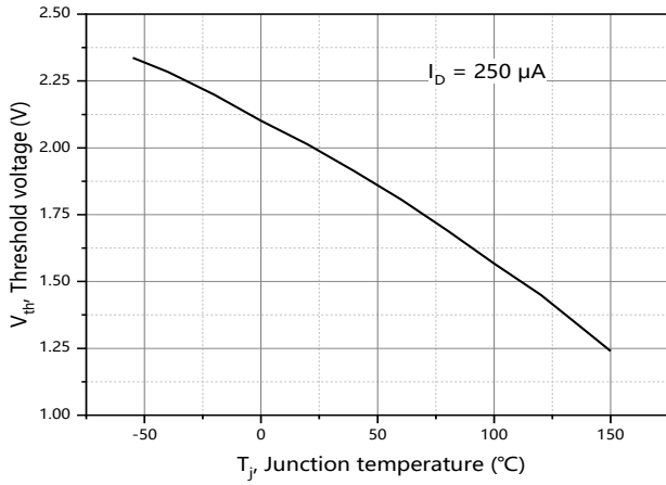
Figure 7. Threshold voltage
