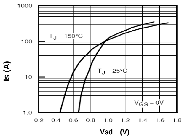
Figure 9. Body-Diode Characteristics
