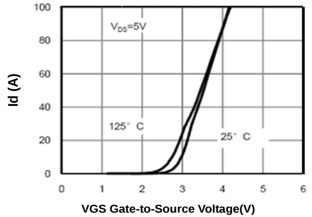
Figure 4. Drain Current
