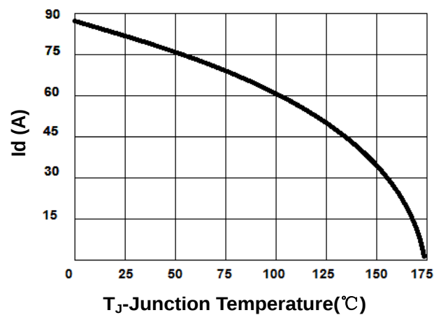
Figure 4. Drain Current
