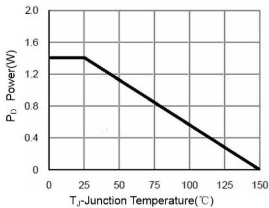
Figure 3 Power Dissipation
