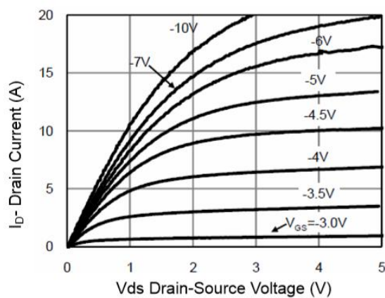
Figure 5 Output Characteristics
