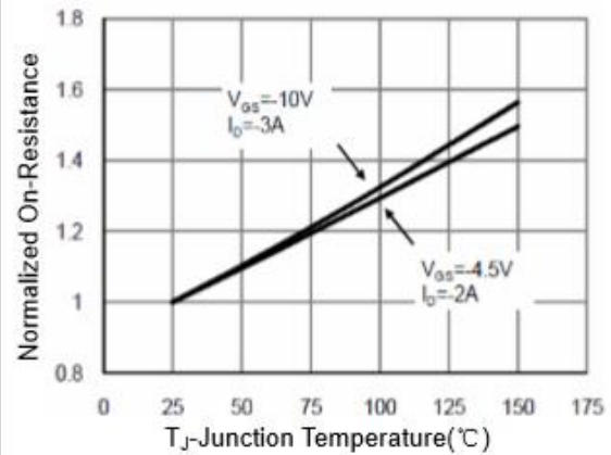
Figure 8 Drain-Source On-Resistance
