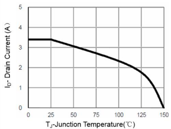
Figure 4 Drain Current
