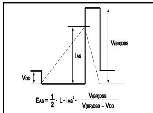
Fig.12 Avalanche Waveform
