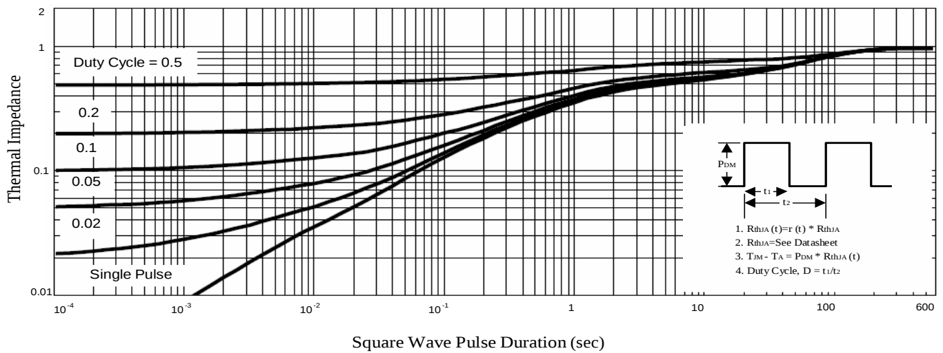
Figure 10. Normalized Thermal Transient Impedance Curve
