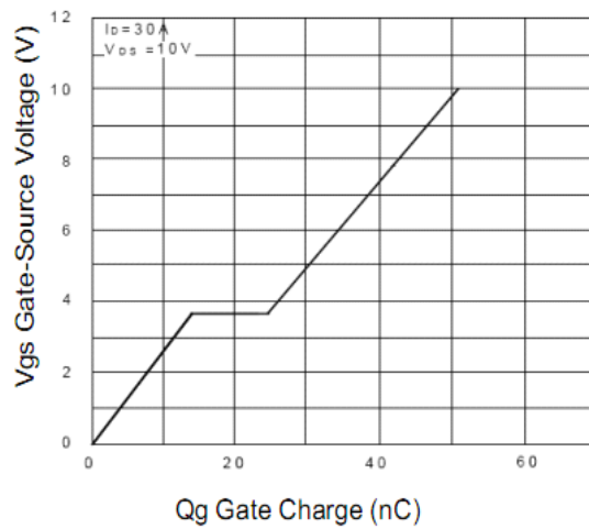
Figure 5 Gate Charge
