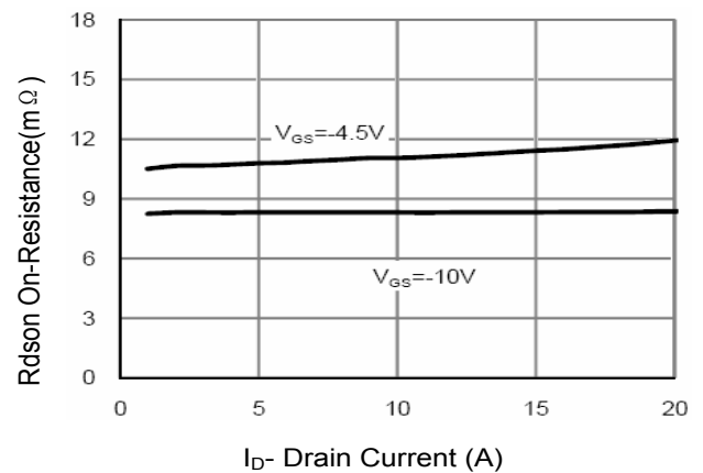
Figure 6 Drain-Source On-Resistance
