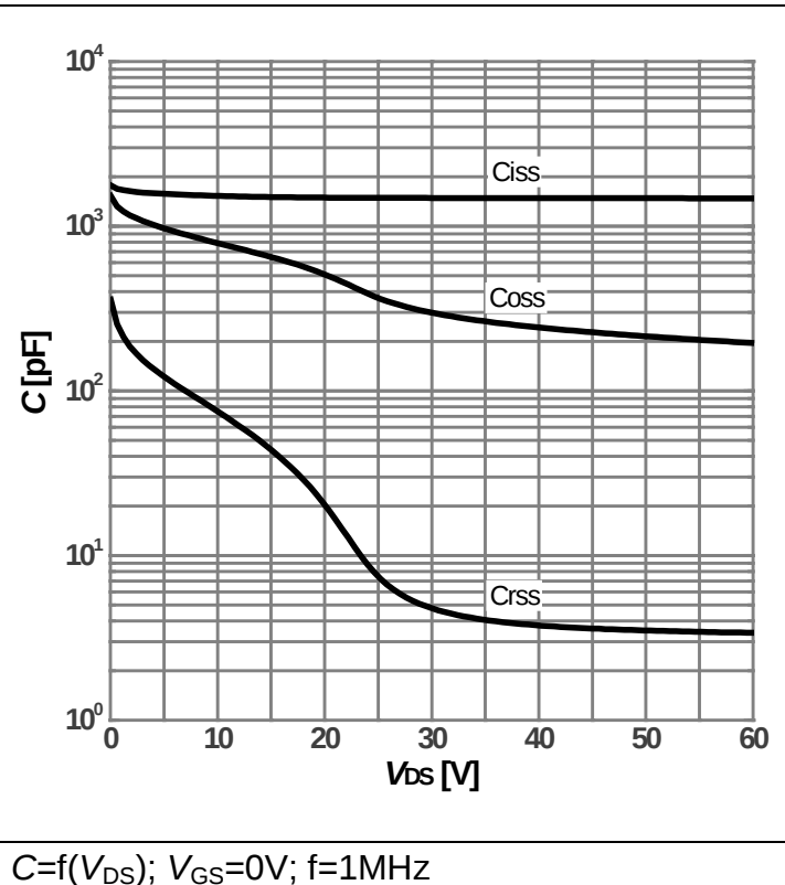
Diagram 13: Typ. capacitances
