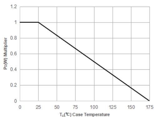
Figure 3. Power Dissipation
