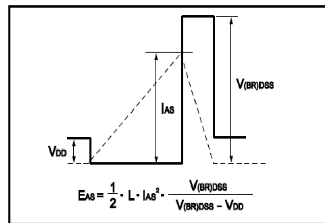
Fig.12 Avalanche Waveform
