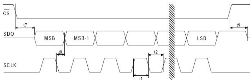
Figure 4-19 SPI 读时序
