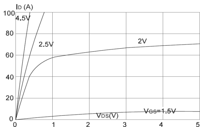
Figure1: Output Characteristics
