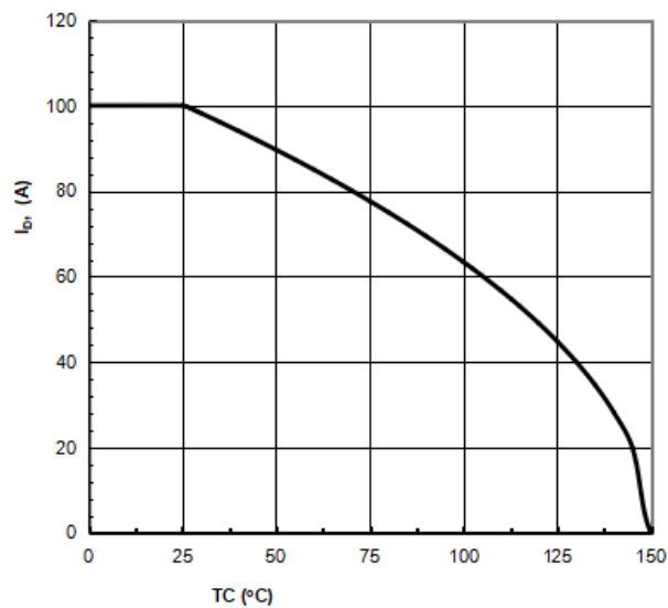
Figure.9: Maximum Drain Current vs. Case Temperature
