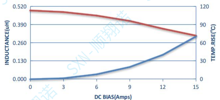
SMTC303018-R47M
