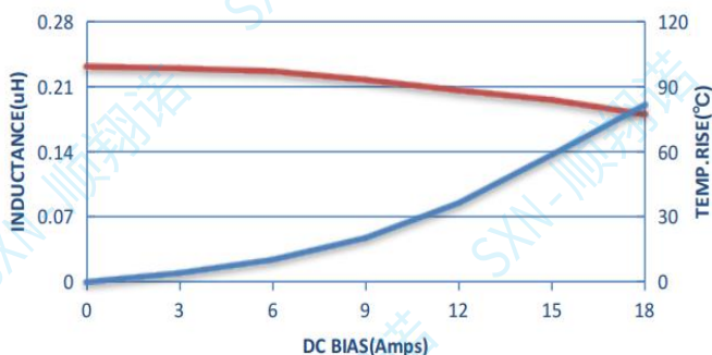
SMTC303018-R22M
