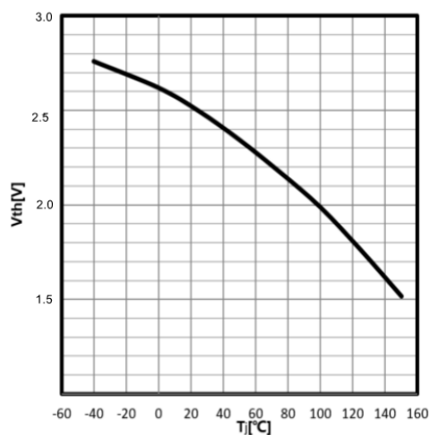
Fig.3 Threshold Voltage V.S Junction Temperature
