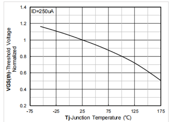
Fig2. V_{GS(th)} Gate -Source Voltage Vs. Tj
