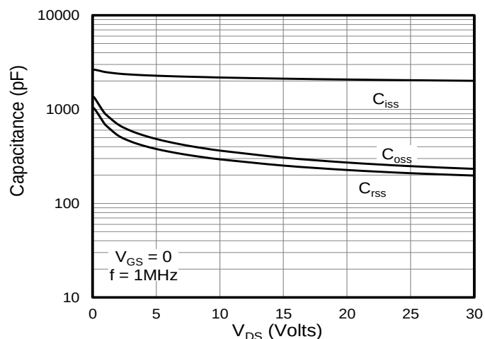
Figure 4: Capacitance Characteristics
