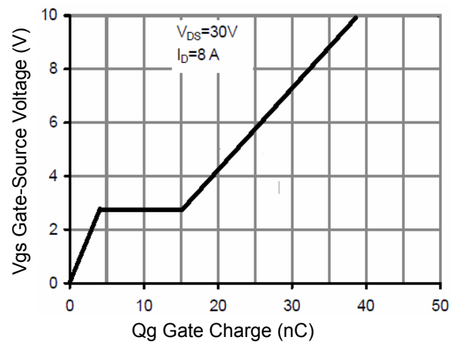
Figure 5 Gate Charge
