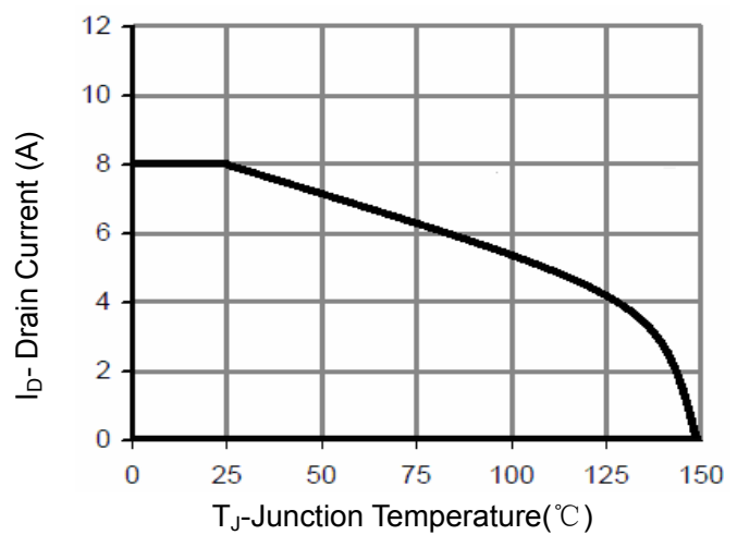
Figure 9 Current De-rating
