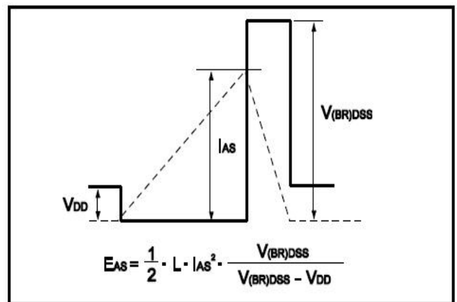
Fig.12 Avalanche Waveform
