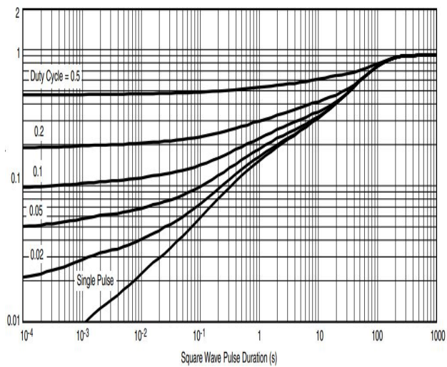
Fig8. Normalized transient thermal impedance
