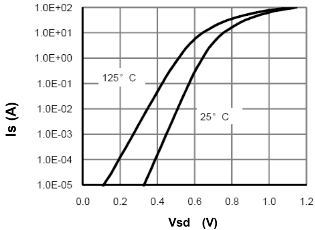
Figure 9. Body-Diode Characteristics
