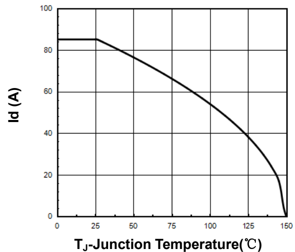
Figure 4. Drain Current
