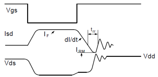
Diode Recovery Test Circuit &amp; Waveforms
