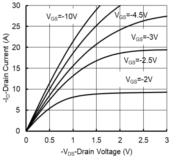
Figure1. Output Characteristics
