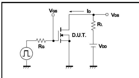
Fig.9 Switching Time Measurement Circuit
