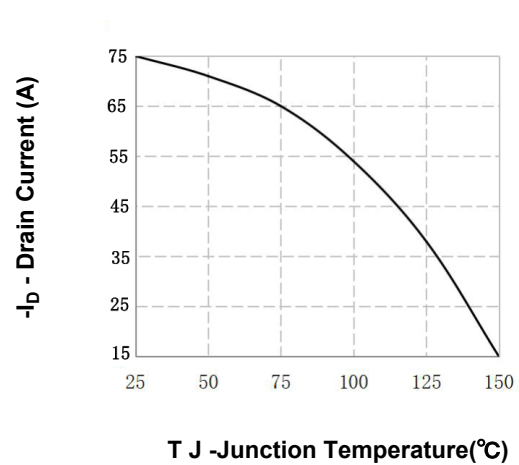
Figure 10. Maximum PContinuous Drain Current vs Case Temperature
