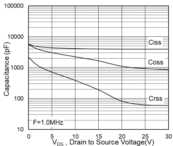
Fig.7 Capacitance
