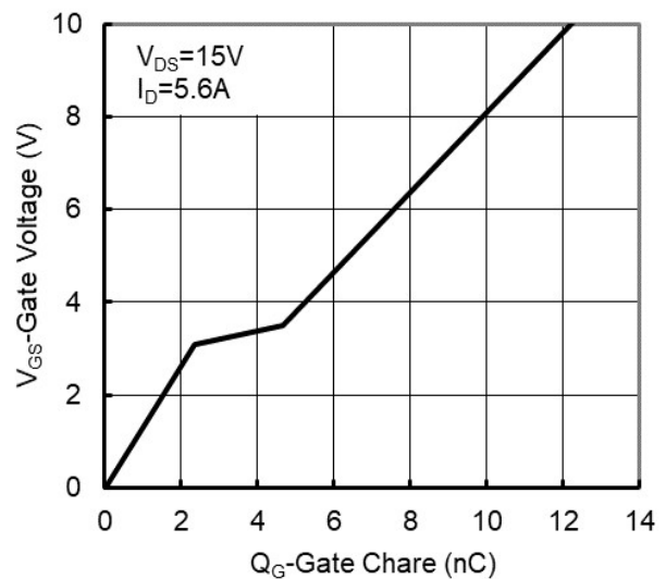
Figure6. Gate Charge
