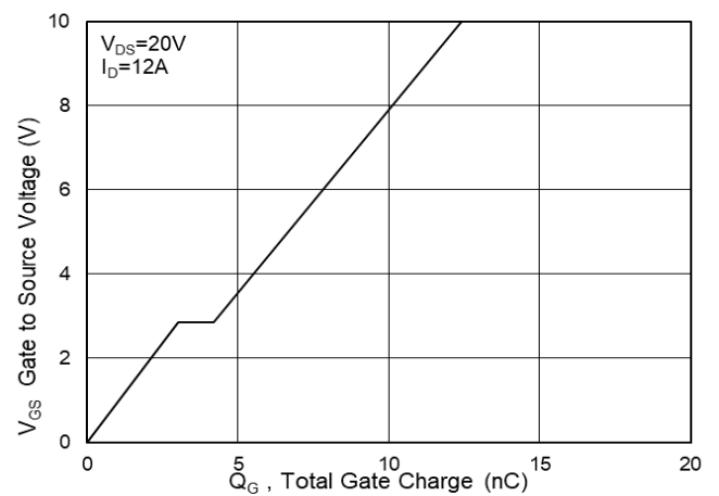
Fig.4 Gate-Charge Characteristics
