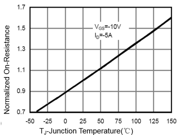
Figure 4 Rdson-Junction Temperature
