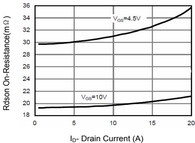
Figure 5 Drain-Source On-Resistance
