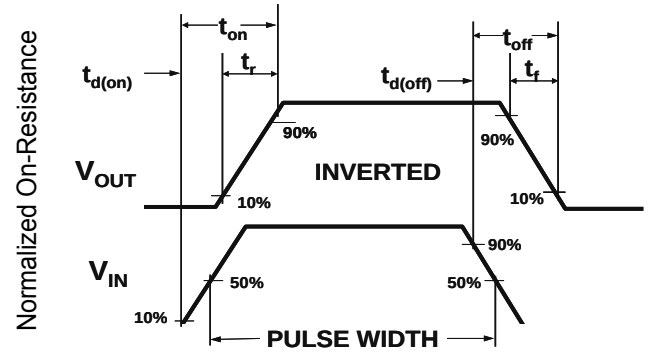
Figure 2: Switching Waveforms
