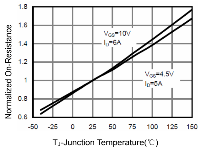
Figure 6 Drain-Source On-Resistance
