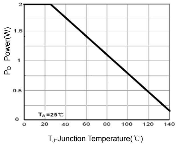
Figure 8 Power Dissipation
