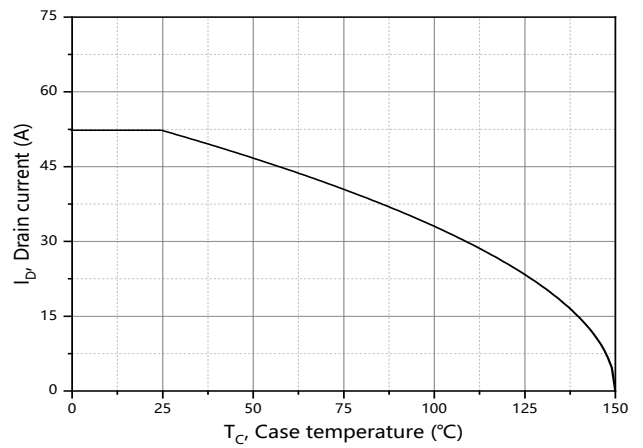
Figure 10. Drain current
