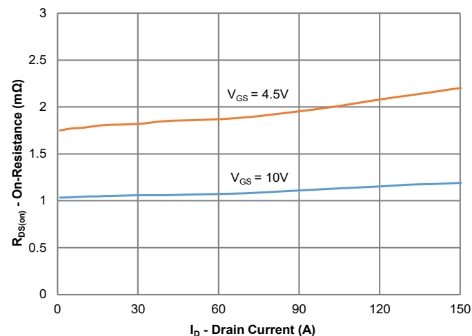
Figure 4: On-Resistance vs. Gate-Source Voltage
