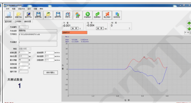
Fig.33 Initial Extraction Force
