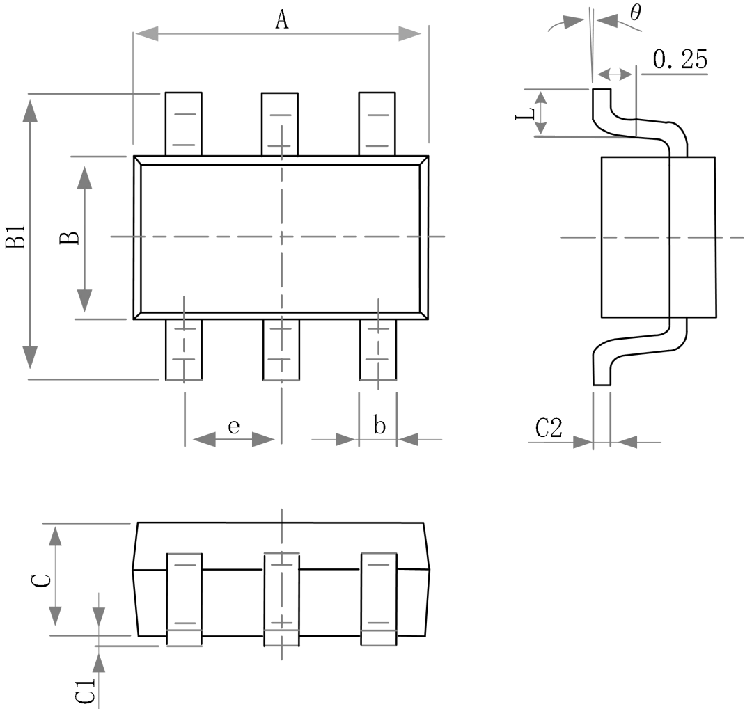
SOT23-6 Package Outlines
