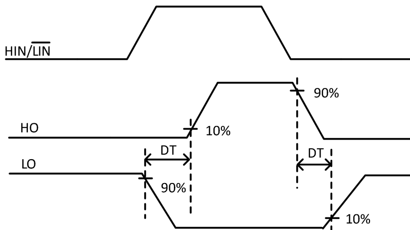
Figure 7. Cross Conduction Prevention Delay Time Waveform Definition
