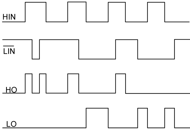
Figure 5. NSG6398 Input and output timing waveform
