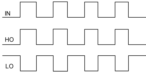
Figure 5. NSG2105 Input and output timing waveform
