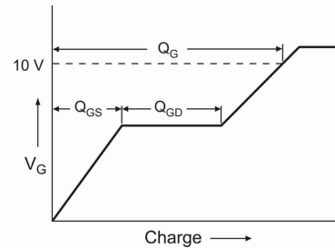
Fig. 17 - Basic Gate Charge Waveform
