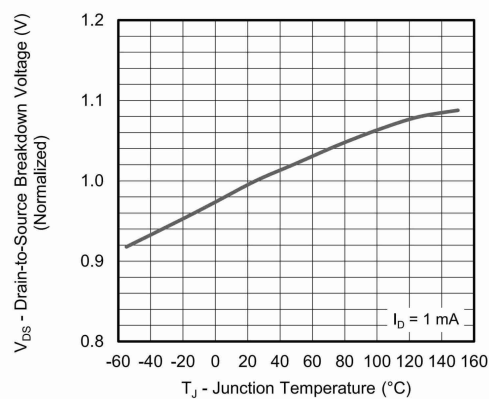
Fig. 11 - Temperature vs. Drain-to-Source Voltage
